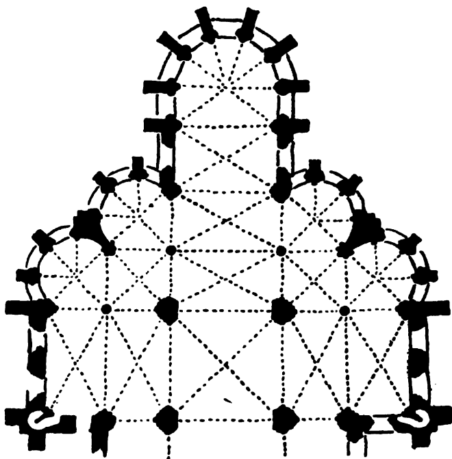
FIG. 70. Church of St. Yved at Braisne, near Soissons.
